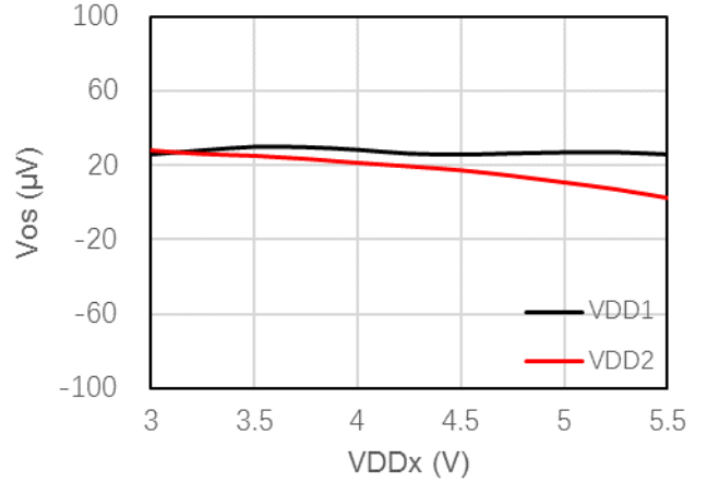
图 7-4 输入失调电压 vs 供电电压 (CA-IS1300G25)
