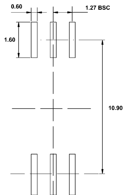
RECOMMENDED LAND PATTERN
